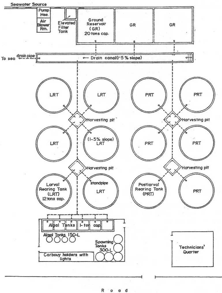
Fig. 11. A sample layout of a prawn hatchery.
